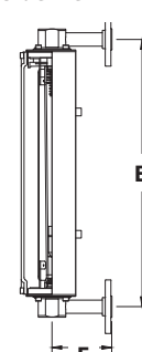
Horizontal Flange Side View
