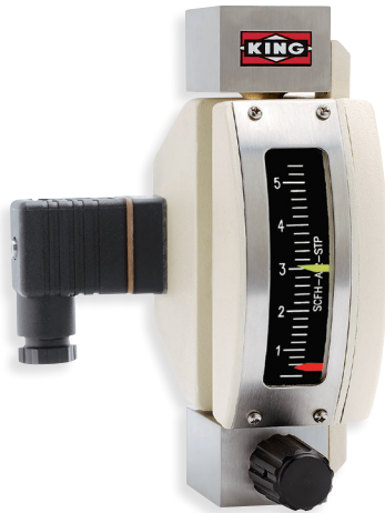
7100 with Inductive Slot Sensor
